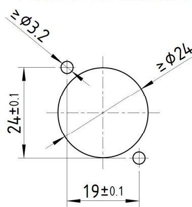
Panel Cut out dimension
