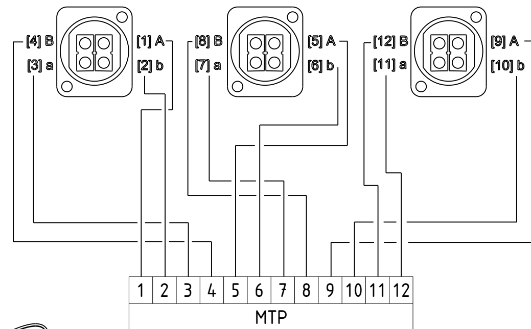
wiring back view
