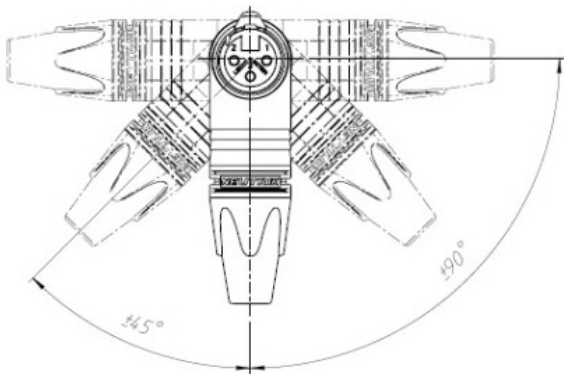
Outlet Positions
