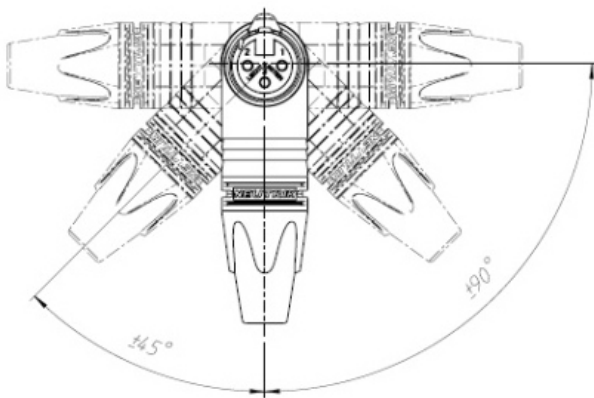
Outlet Positions
